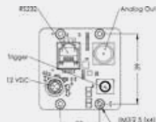
Analog interface
