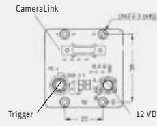
CameraLink interface
